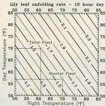
Figure 1. Isopleth plots of lily leaf unfolding rates for 1A) a 10-hour day and 1B) an 11-hour day and 13-hour night.
